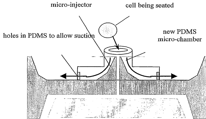
Fig. 19. New design that uses a top PDMS layer, forming the \mu -chamber and allowing for fluid venting and suction. The bottom PDMS acts as cavity backfill.
